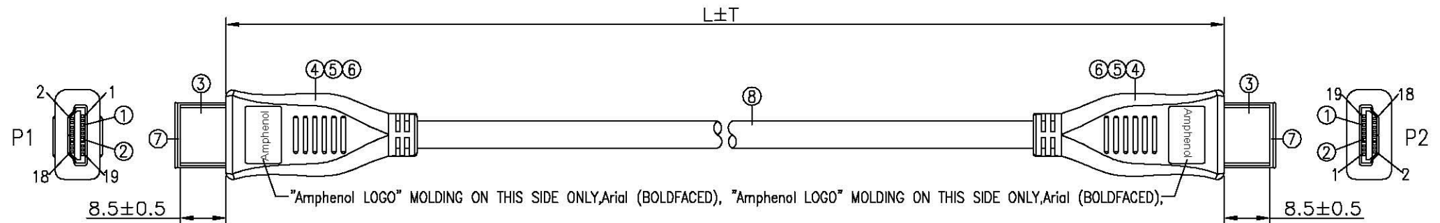
HDMI 19PIN MALE(MOLDING TYPE)
